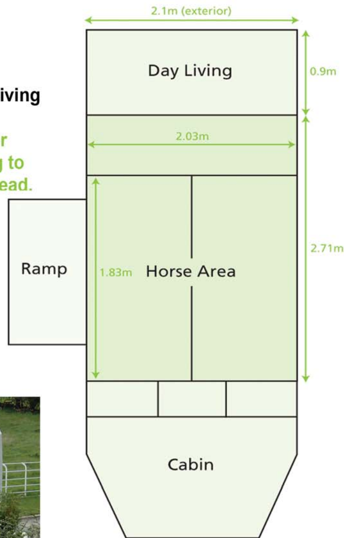
All models have same internal dimensions in horse area. Diagram shows Day living in X and XS models.
